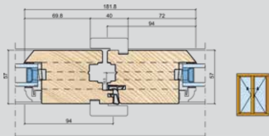
French door
