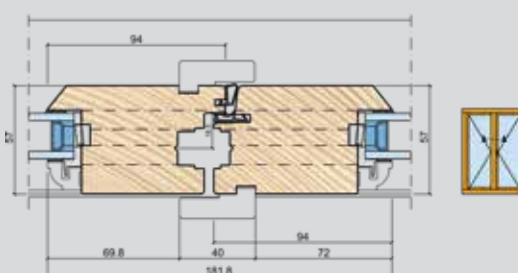
French door
